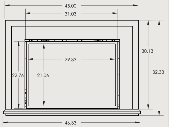
Extra Large Gas Insert
