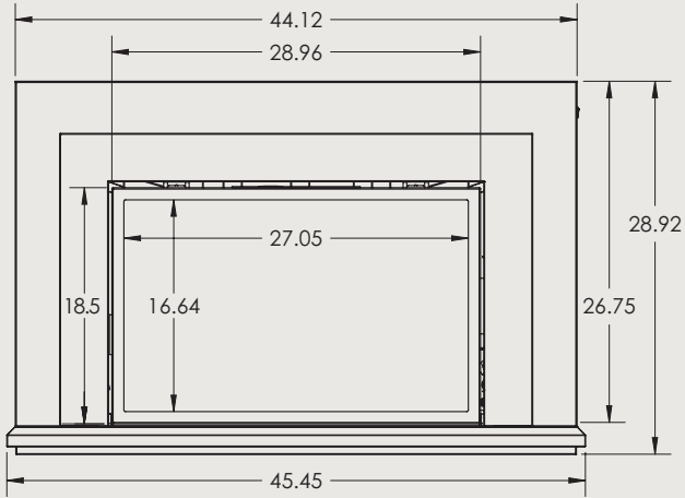
Large Gas Insert
